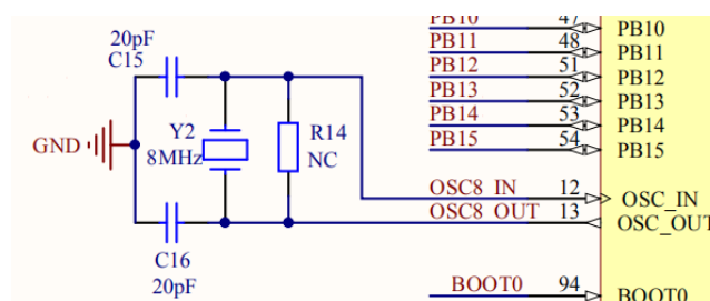
Figure 2 Crystal Oscillator Circuit
